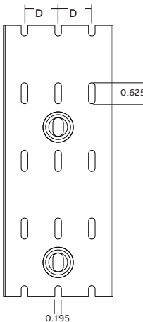
Pattern for 2", 2 1/2", 3", 4" & 6"
