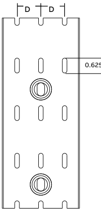
Pattern for 2", 2 1/2", 3", 4" & 6"
