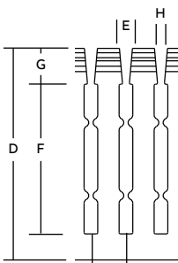
3", 4" and 5" heights
