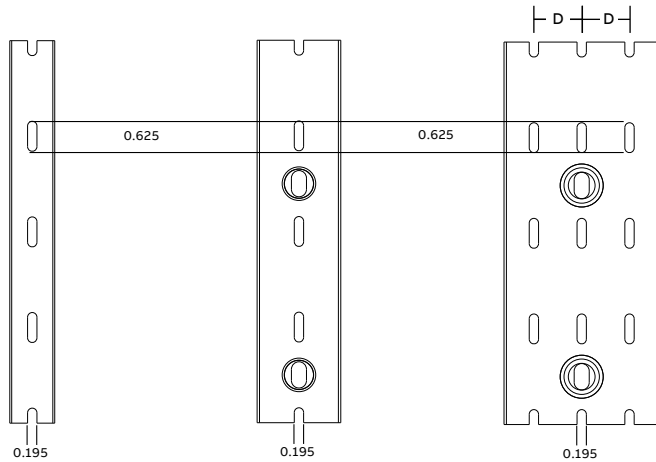
Pattern for 3/4" & 1"
