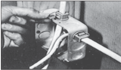
Snap captive locking wedge into fitting's cavity.
